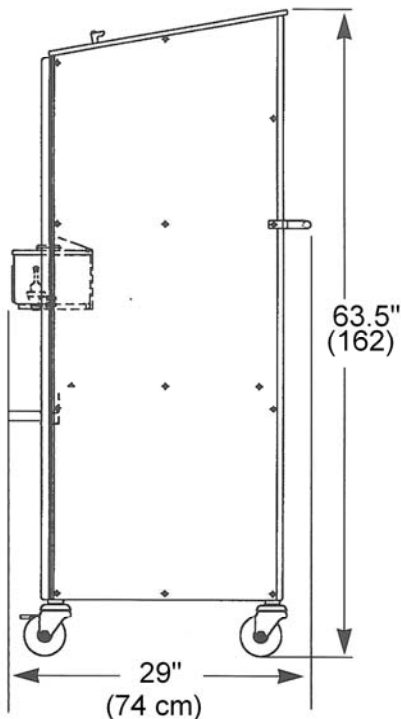
SIDE VIEW Outside Dimensions
